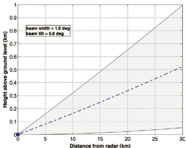
FIG. 4. Beam height AGL for a small (1-m antenna) short wavelength (X-band) radar. The shaded region is the coverage by the 1.8° beam at 0.9° elevation angle. The dotted line is the center of the beam. At this lowest tilt, the entire beam is below 1 km over a 30-km range.
