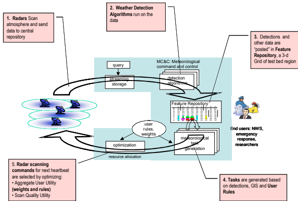
Fig. 2. Schematic showing the flow of data and control within IP1.
