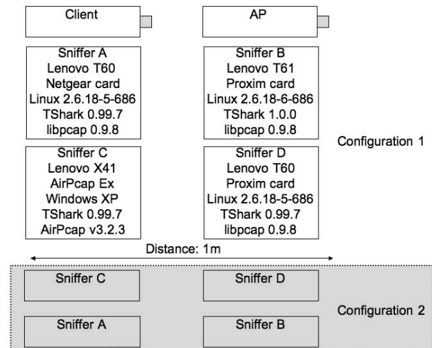
Fig. 1. Setup for the measurements
