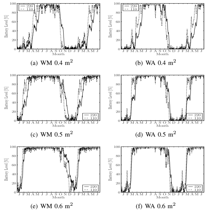
Fig. 10. Battery level in percentage capacity for two locations each with two battery capacities and three solar panel areas. Battery capacity is presented in percent capacity relative to the battery size (110 or 220 Ah). Panel size is 0.4, 0.5 or 0.6 m 2 .
