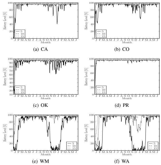
Fig. 9. Battery level in percentage capacity relative to a 110 Ah battery for six locations with a fixed 110 Ah battery capacity.
