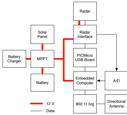
Fig. 1. OTG prototype hardware architecture.
