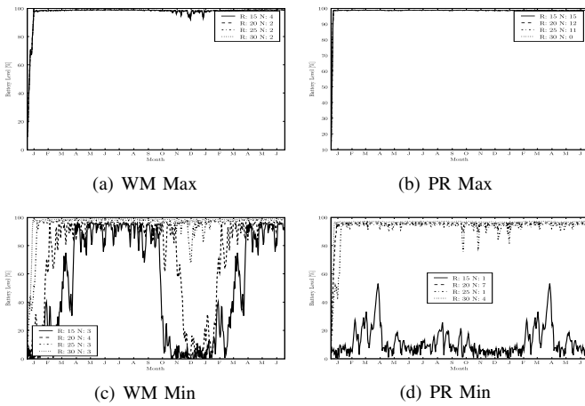
Fig. 13. Battery level of the nodes with the maximum and minimum cumulative sum battery levels.
