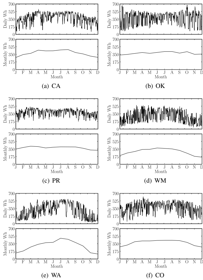
Fig. 6. Daily and monthly mean estimated solar power generation in Wh for the six sites in the location experiment.
