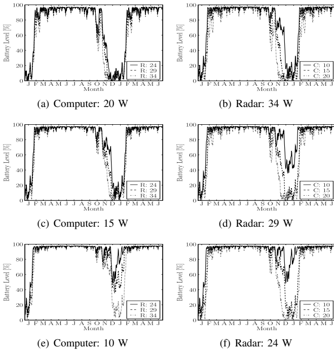
Fig. 11. Battery level in percentage capacity relative to a 110 Ah battery for 9 different system configurations.
