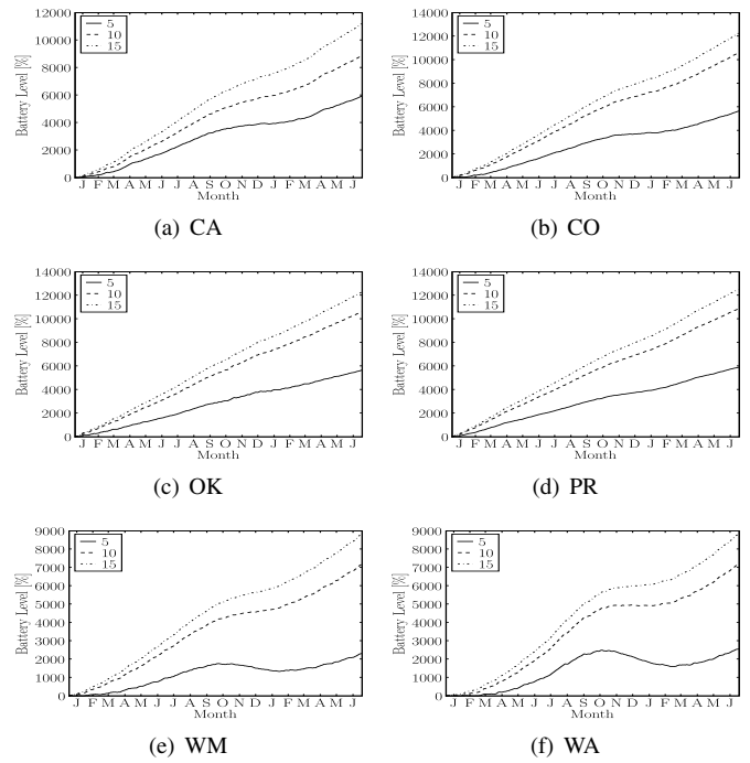
Fig. 7. Battery level in percentage capacity relative to a 110 Ah battery. Nodes were simulated with an unlimited battery, 0.5 m 2 panel and three different scan interval times: 5, 10 and 15 minutes.
