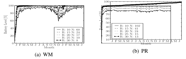
Fig. 12. Average battery level for WM and PR, node separation was been varied from 10 - 30 km. The number of nodes in each network is indicated in the legend of the figure.
